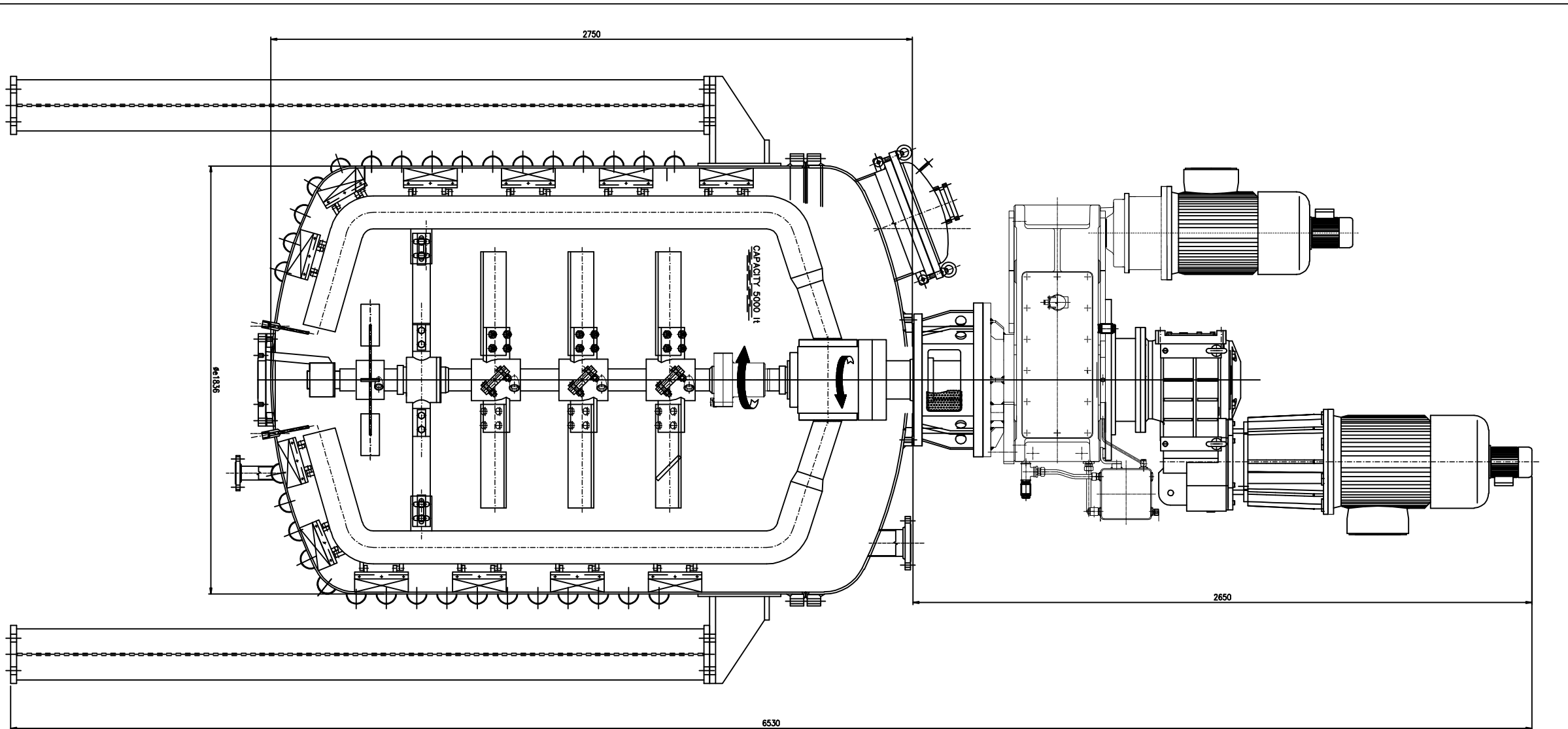
N°1 COUNTER ROTATING MIXING UNIT 5000 Lt
